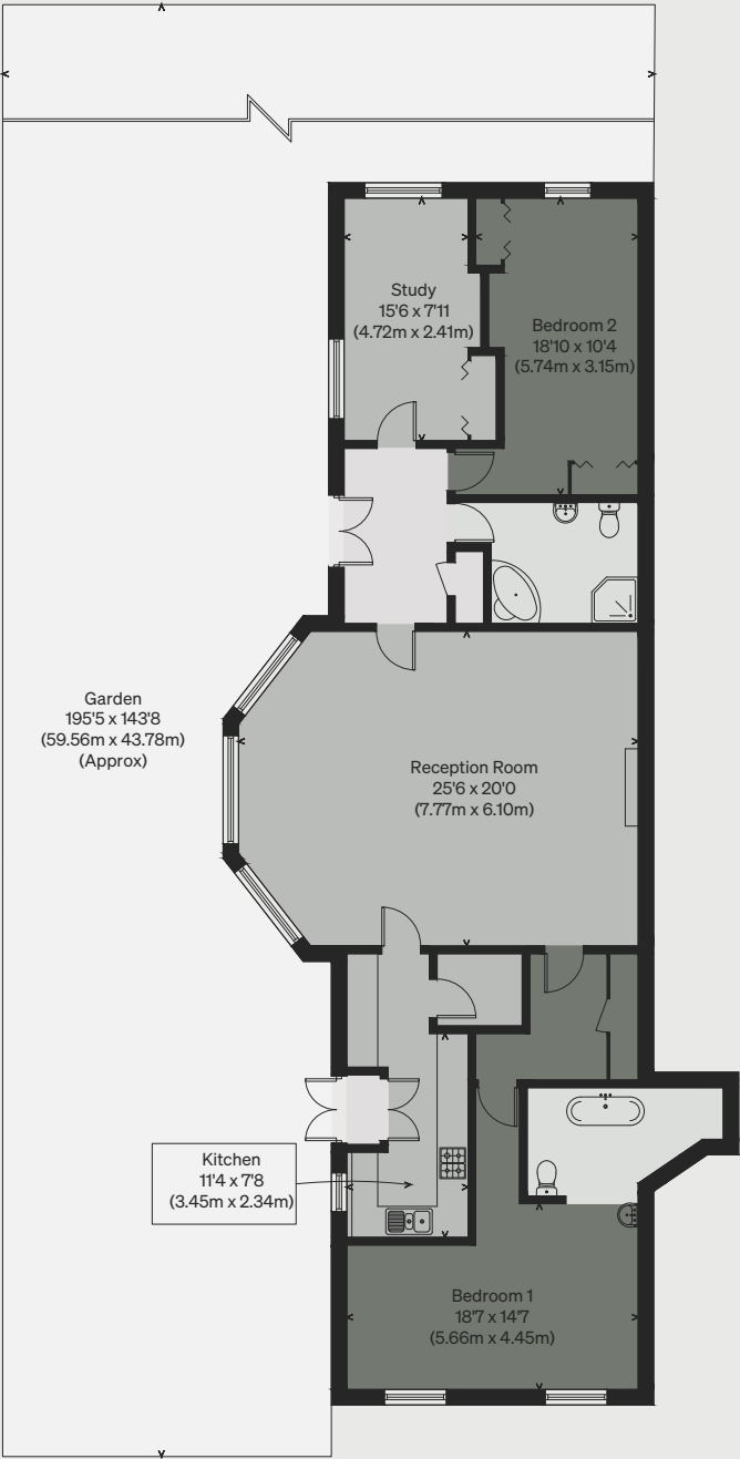
GROUND FLOOR
