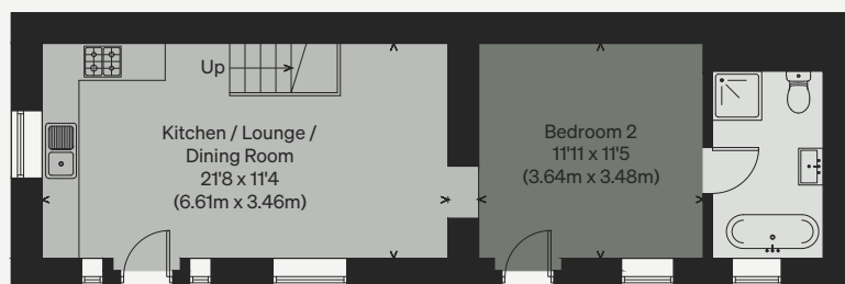
ANNEXE - GROUND FLOOR
