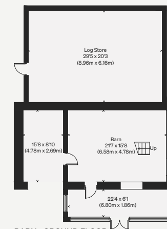
BARN - GROUND FLOOR (Not Shown In Actual Location / Orientation)
