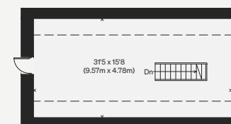
BARN - FIRST FLOOR
