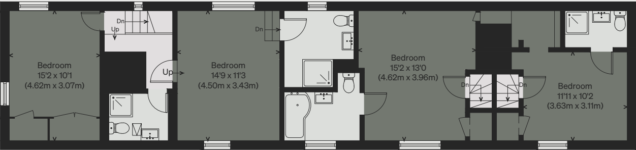
FIRST FLOOR
