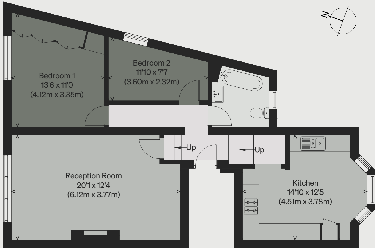
RAISED GROUND FLOOR
