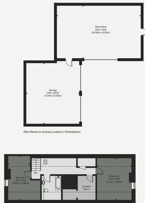
SECOND FLOOR
