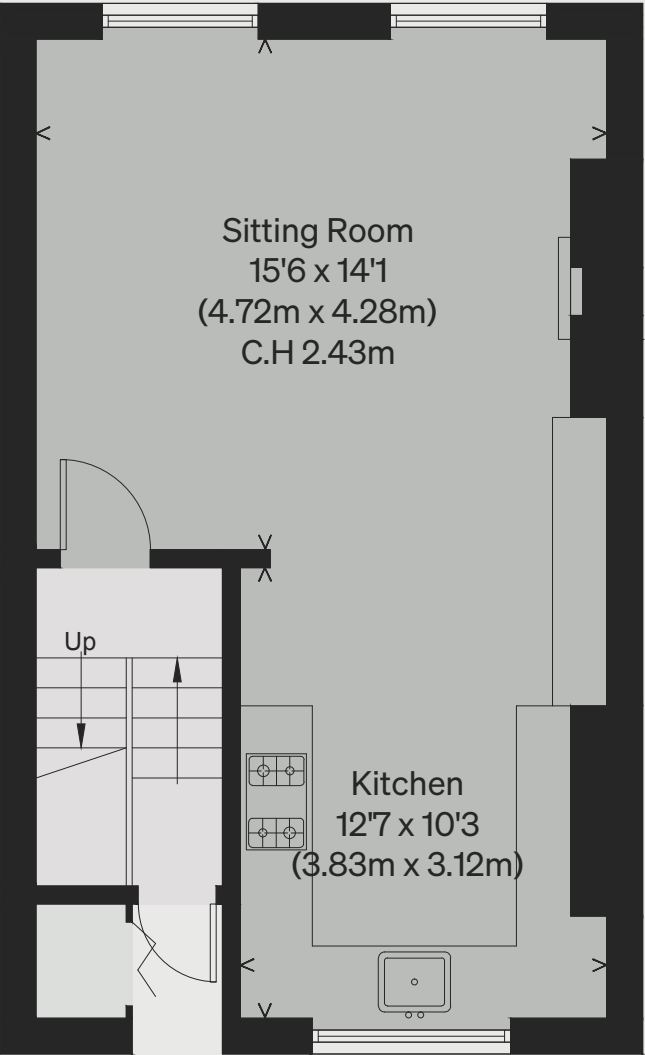
SECOND FLOOR
