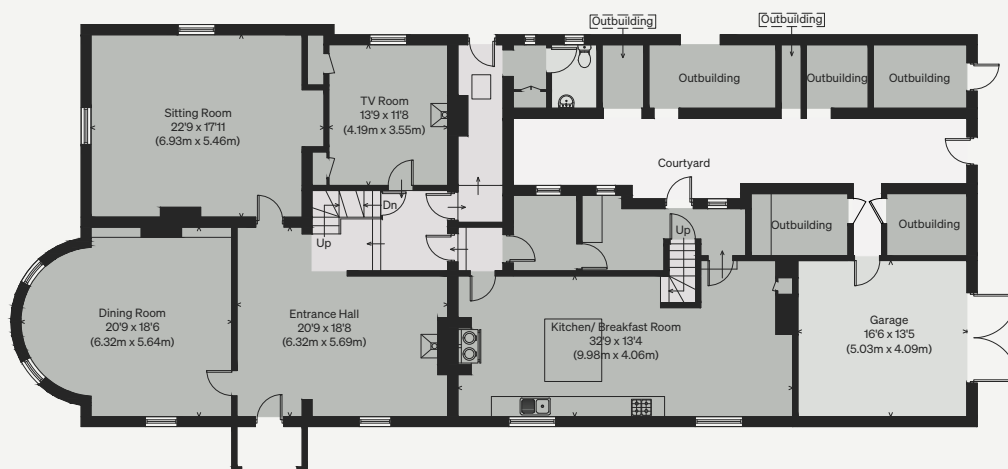
GROUND FLOOR
