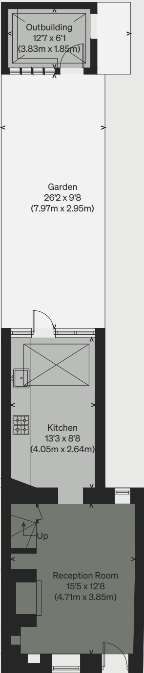
GROUND FLOOR
