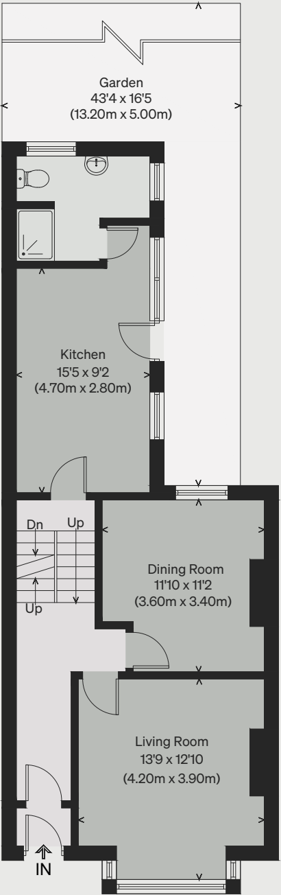
GROUND FLOOR
