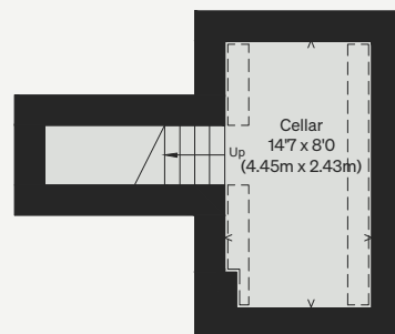
CELLAR
