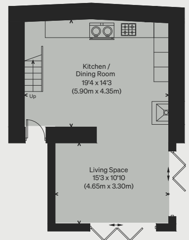
COTTAGE - GROUND FLOOR
