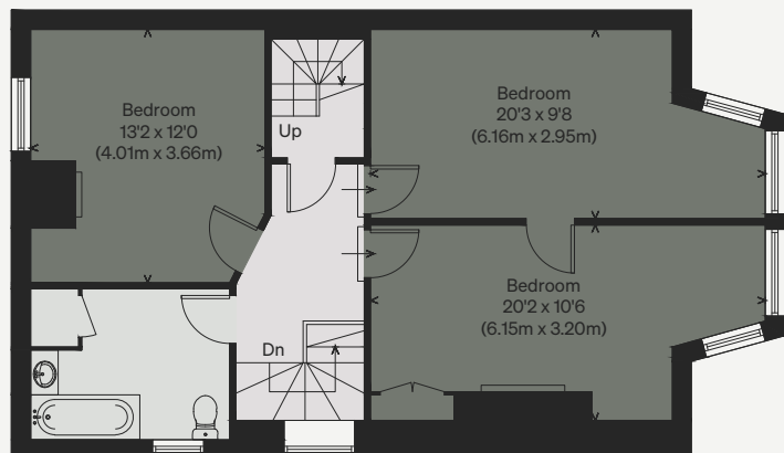
SECOND FLOOR
