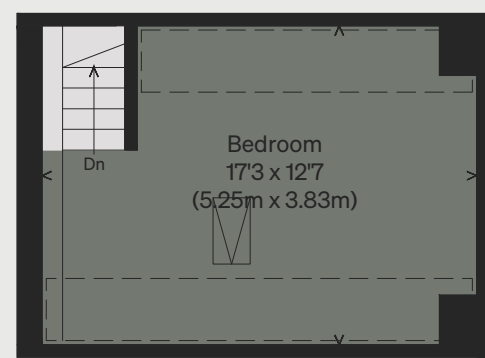
SECOND FLOOR / ROOF ROOM
