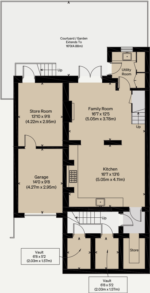
GROUND / LOWER GROUND FLOOR
